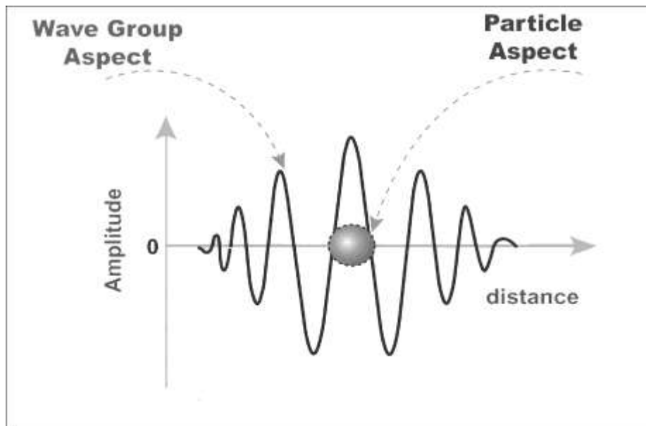
Figure A.2a. The de Broglie particle/pilot wave concept of the 1920's, for which he won a Nobel Prize, proposed that every particle had a group wave envelope enclosing it and moving at the particle's velocity. [however, faster than EM-light, c , unseen pilot waves of the physical vacuum move through the group from left to right at velocity v_w > c ].
