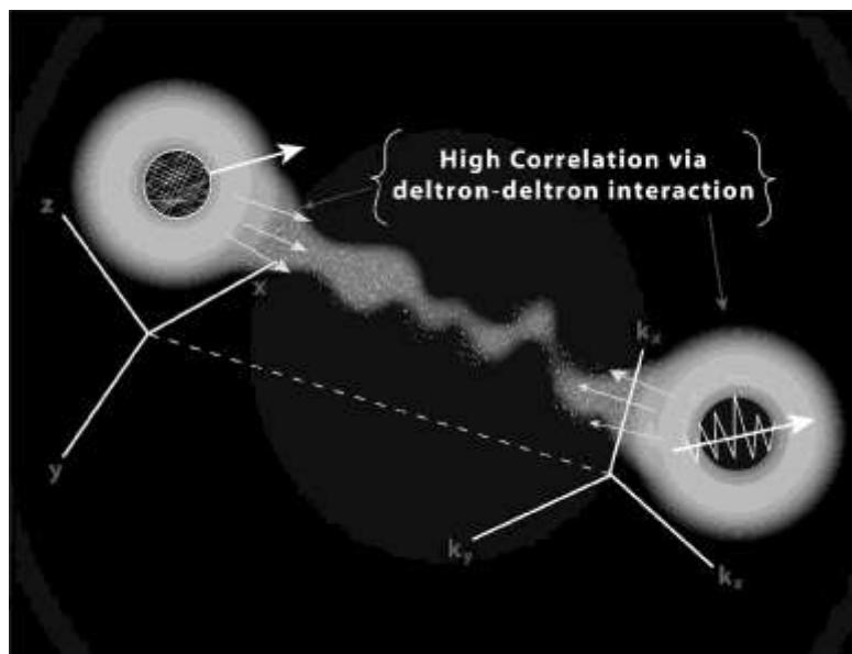
Figure 4. Illustration of how deltron-deltron coupling allows the two unique levels of physical reality to interact with each other.
