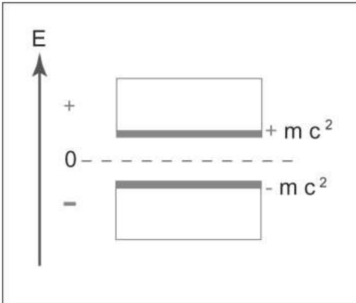
Figure A.1. Schematic energy spectrum associated with the Dirac Equation.
