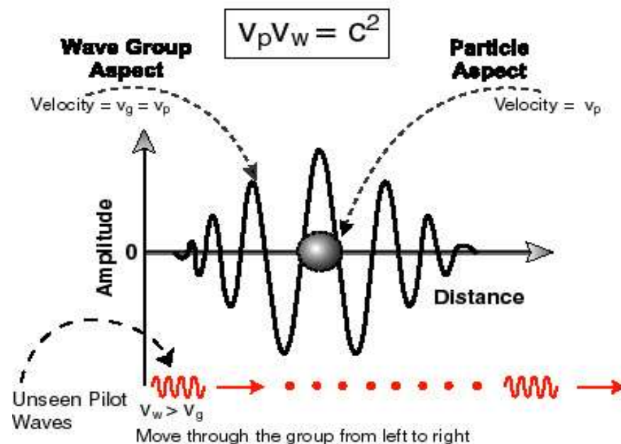
Figure A.2.b. Schematic drawing of true pilot waves.
