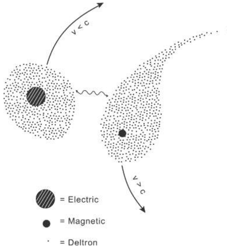
Figure A.3. A higher dimensional level of substance, labeled deltrons, falling outside the constraints of relativity theory and able to move at velocities greater than and less than c , acts as a coupling agent between the electric monopole types of substance and the magnetic monopole types of substance to produce both electromagnetic (EM) and magnetoelectric (ME) types of mediator fields exhibiting a special type of "mirror" principle relationship between them.
